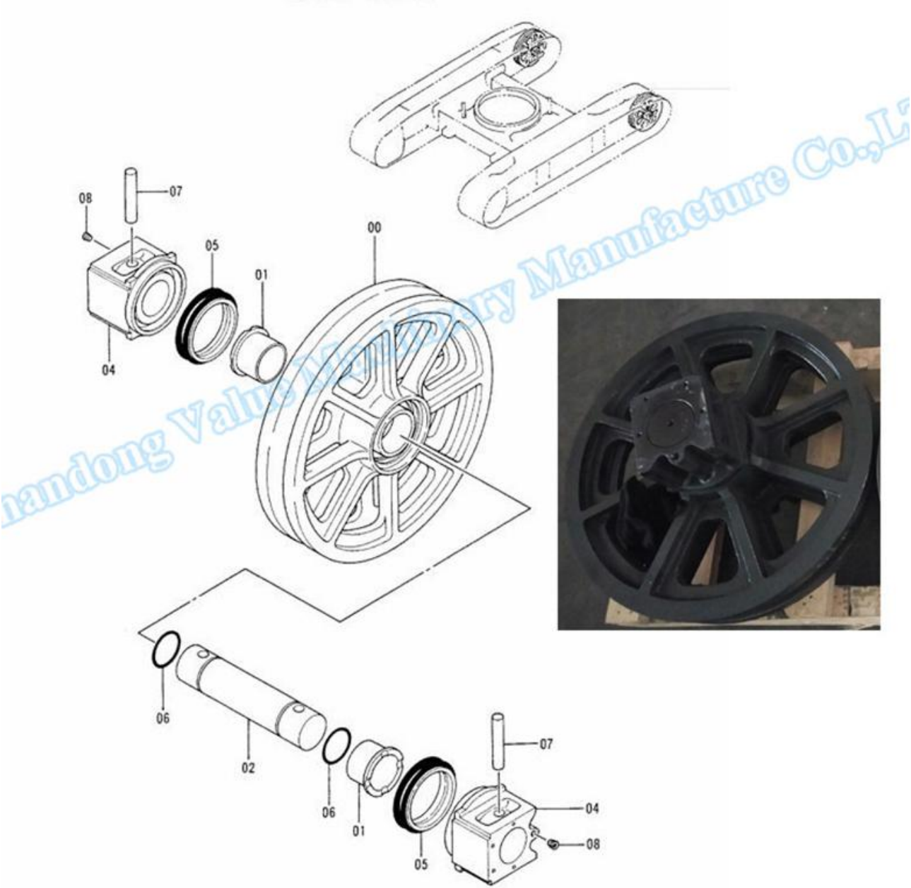
FRONT IDLER
